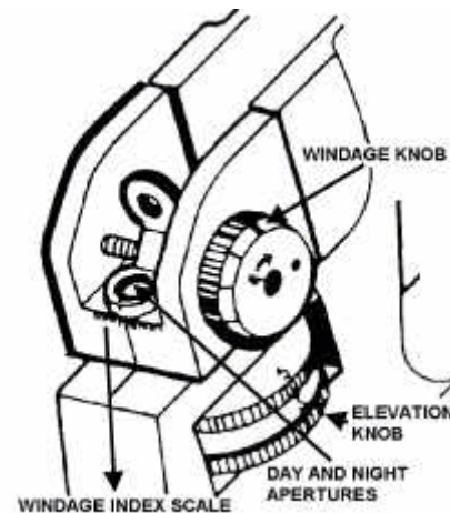
Figure 9-4. Rear Sight.
